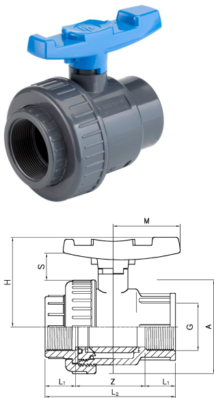
Single union safeblock B.S.P. PVC-U Ball valve with threaded sockets G
