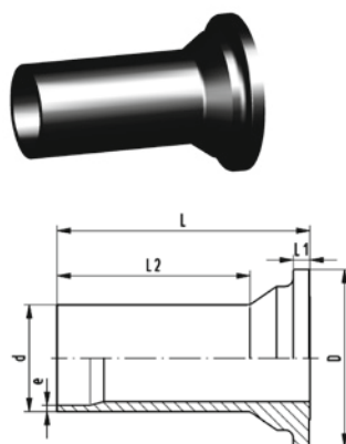
ecoFIT Valve end 546 and 543 (G44) PE100 With butt fusion spigot long SDR17,6 metric
